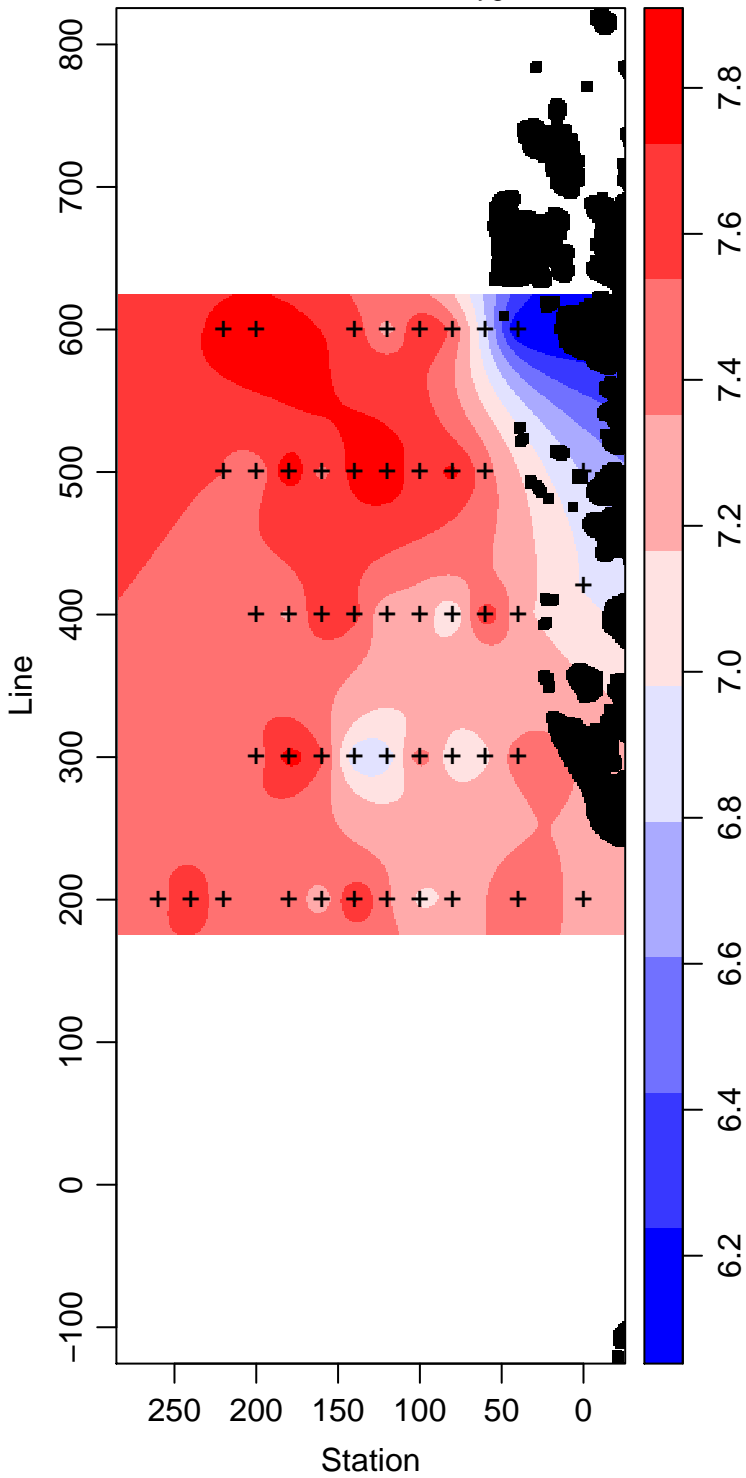
LMG08-01_70_Dissolved.Oxygen ml L -1
