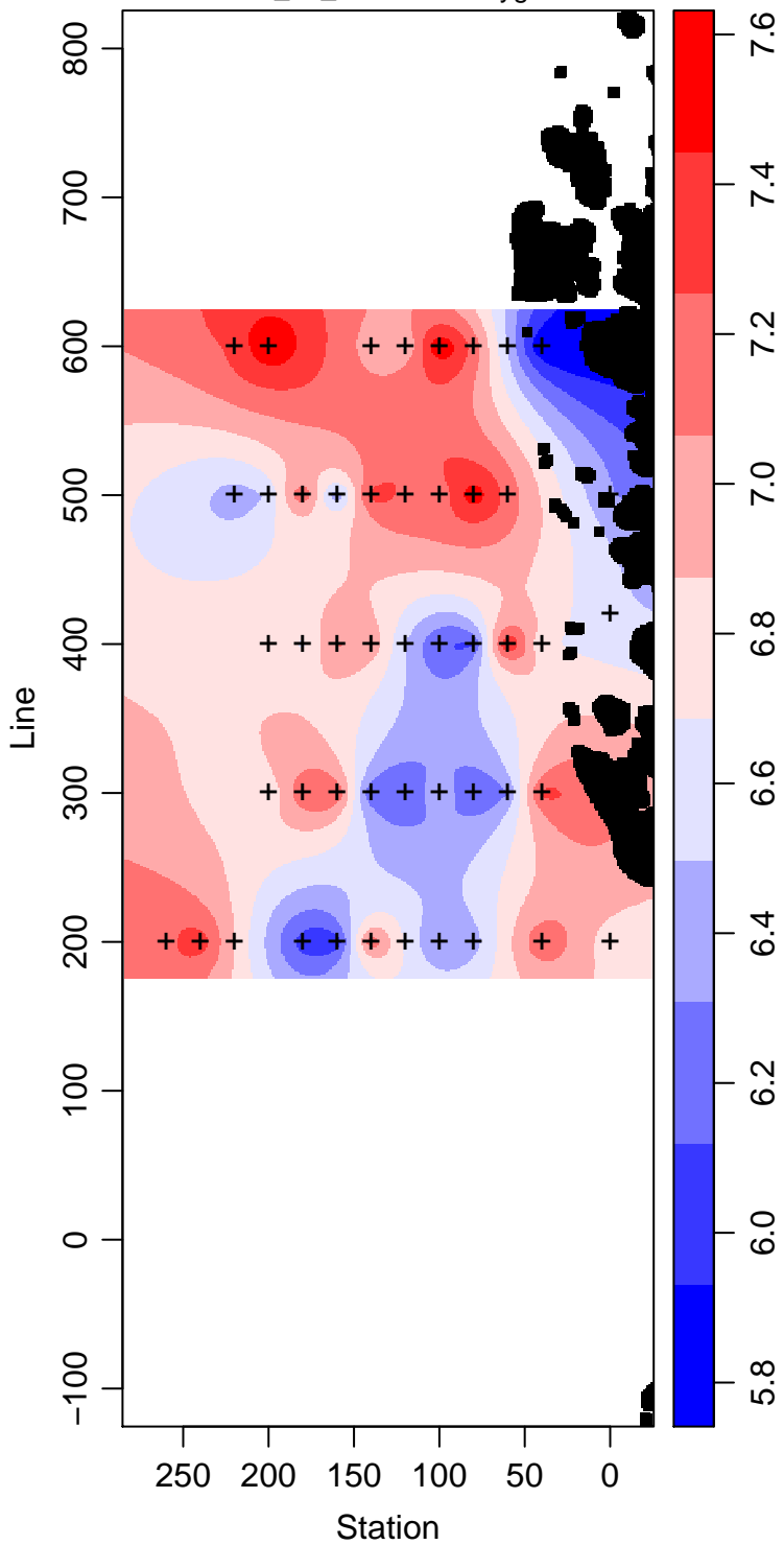
LMG08-01_90_Dissolved.Oxygen ml L -1
