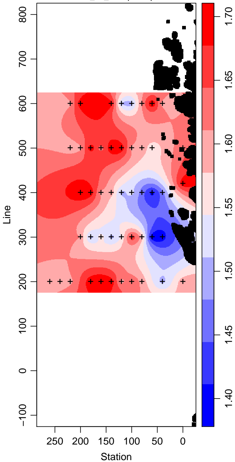
LMG08-01_15_Phosphate \mu\text{ mol L}^{-1}
