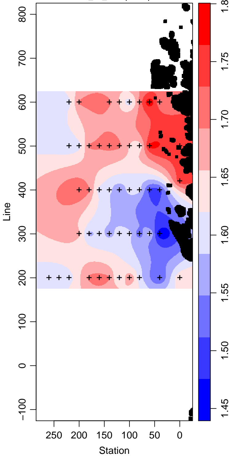
LMG08-01_25_Phosphate \mu\text{ mol L}^{-1}
