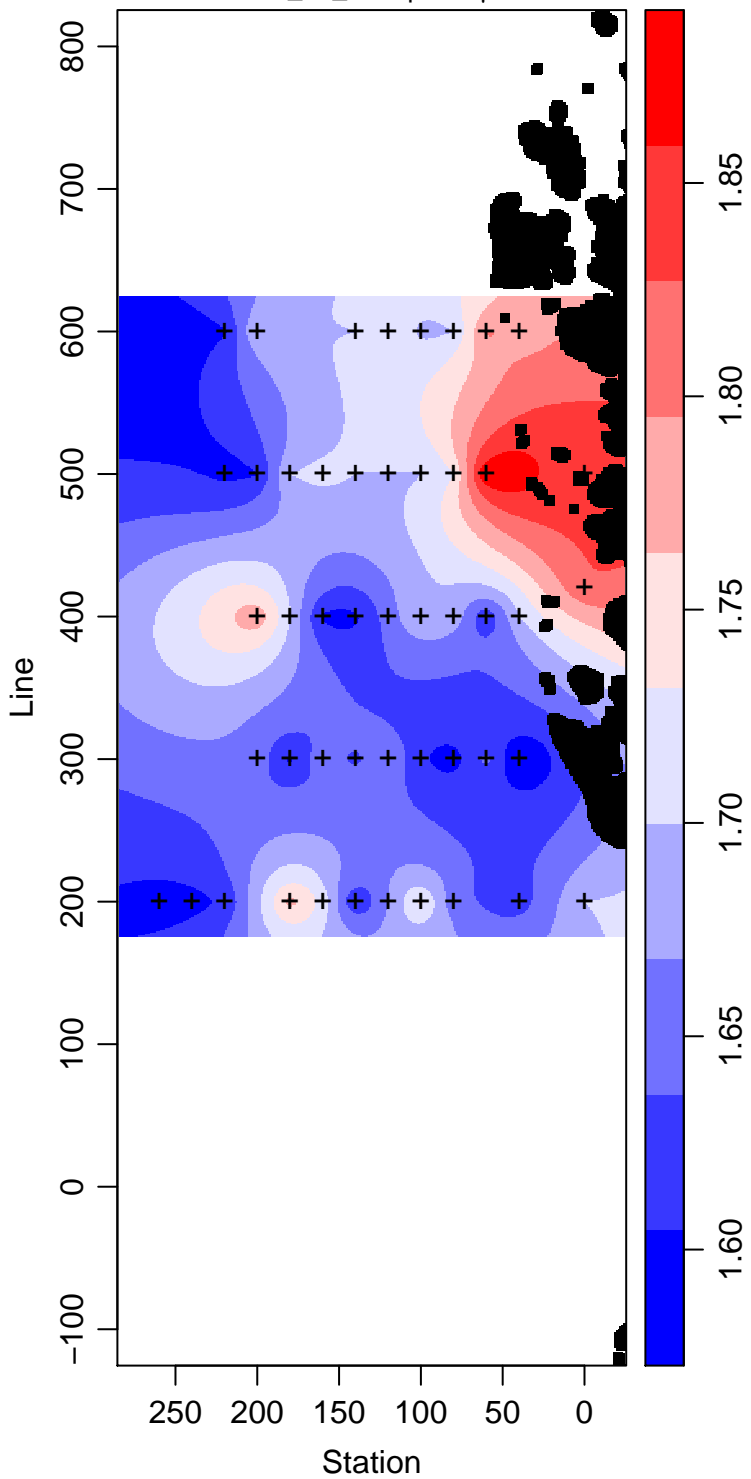
LMG08-01_35_Phosphate \mu\text{ mol L}^{-1}
