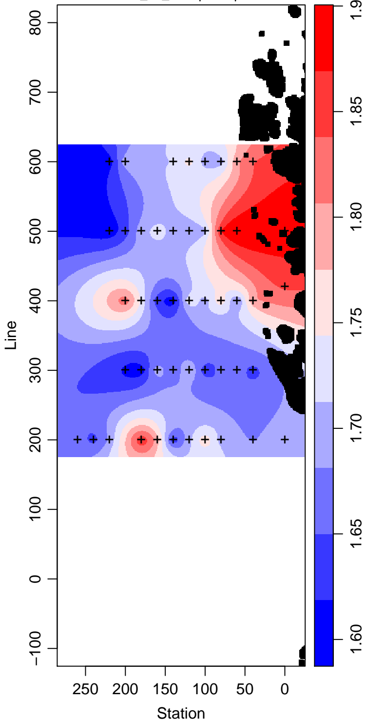
LMG08-01_40_Phosphate \mu\text{ mol L}^{-1}
