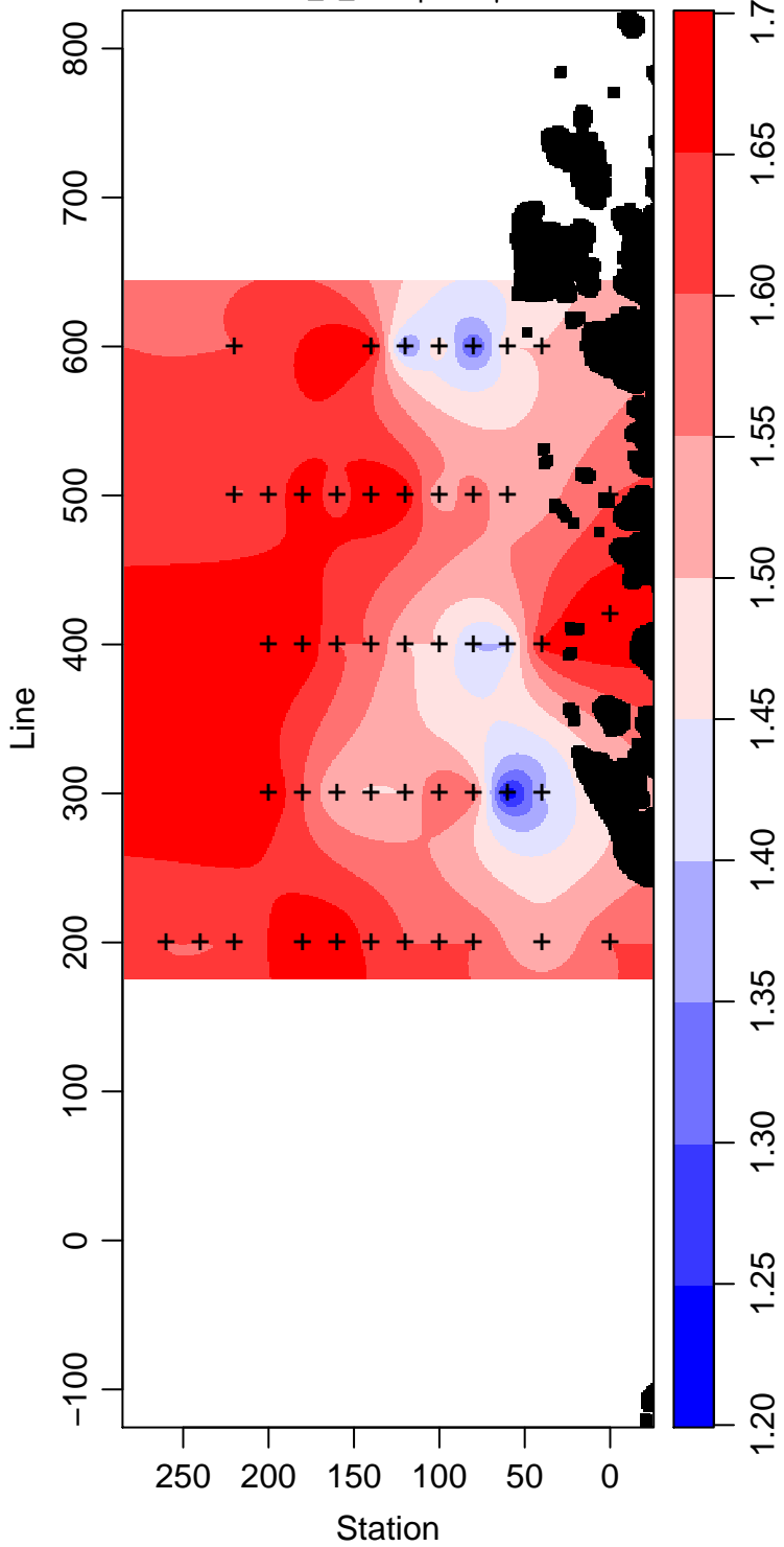
LMG08-01_5_Phosphate \mu\text{ mol L}^{-1}
