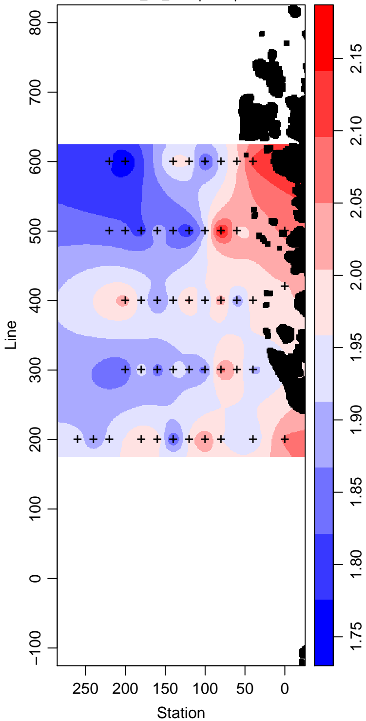
LMG08-01_70_Phosphate \mu\text{ mol L}^{-1}
