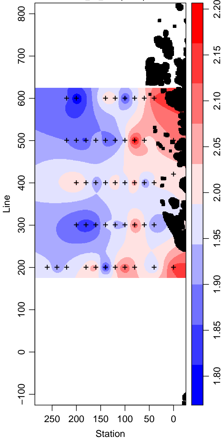
LMG08-01_75_Phosphate \mu\text{ mol L}^{-1}
