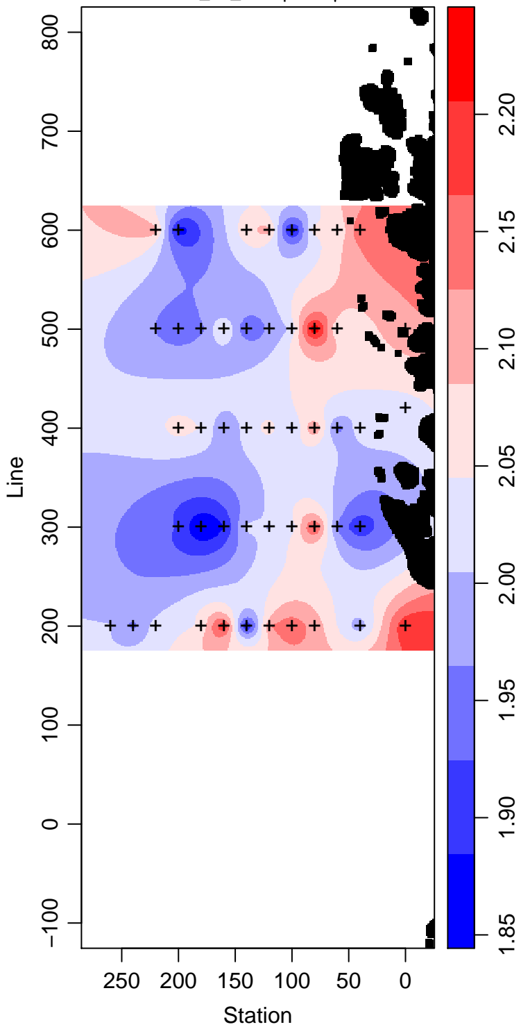
LMG08-01_85_Phosphate \mu\text{ mol L}^{-1}
