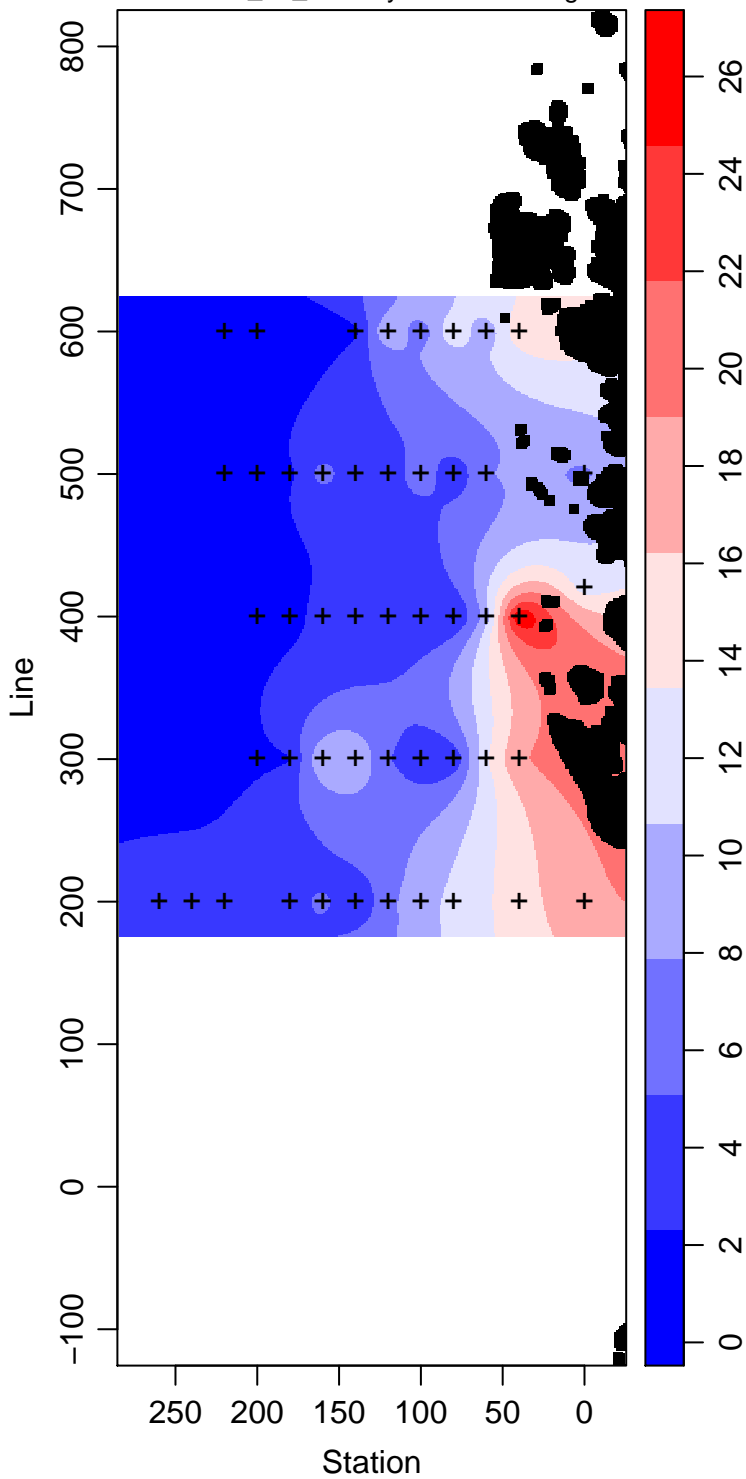
LMG08-01_15_Primary.Production mg m -3
