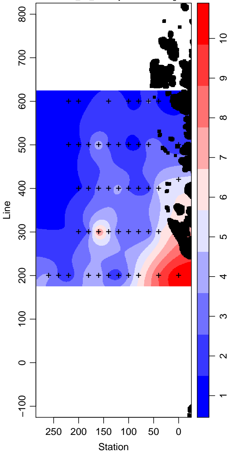
LMG08-01_40_Primary.Production mg m -3
