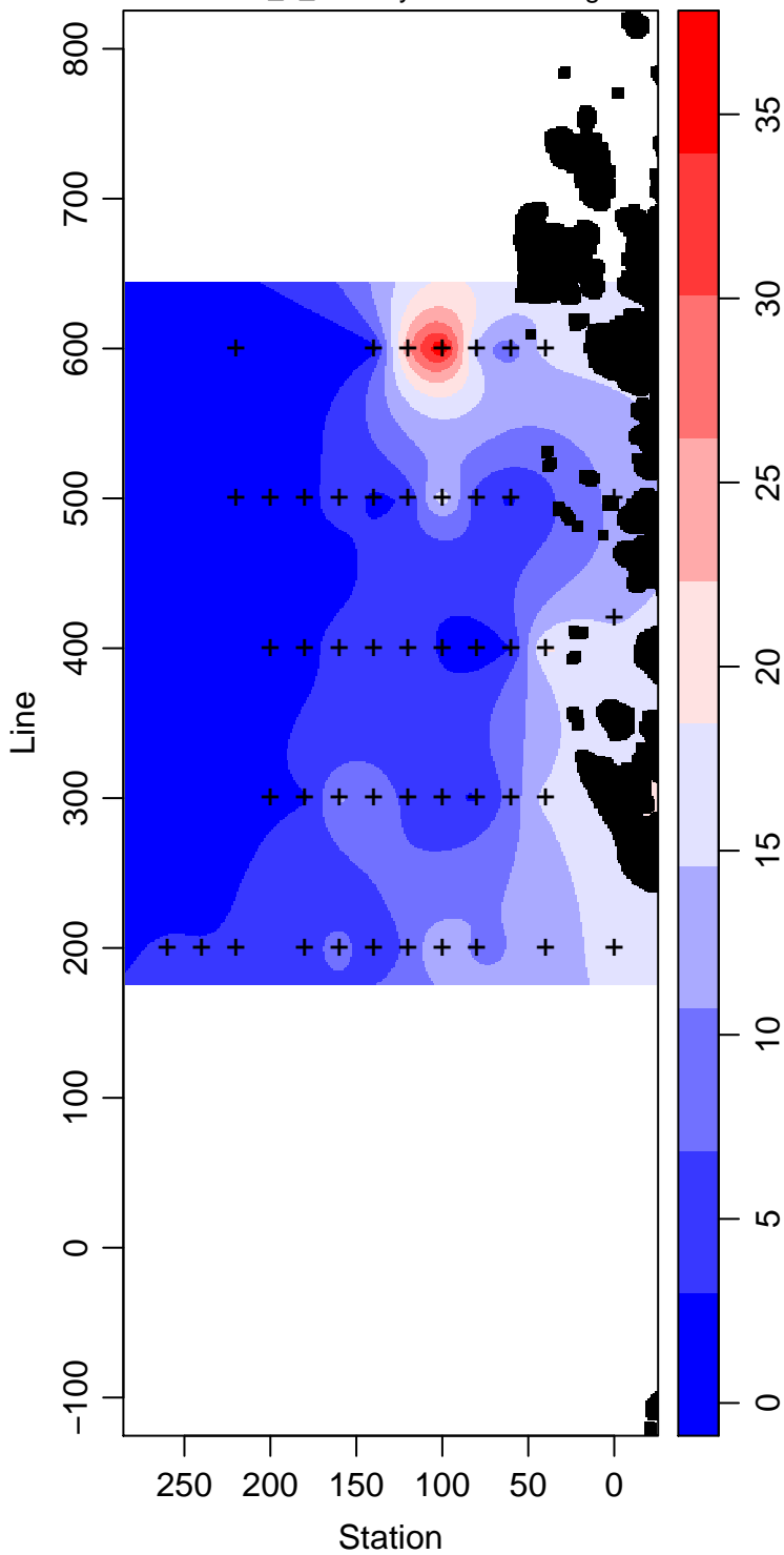
LMG08-01_5_Primary.Production mg m -3
