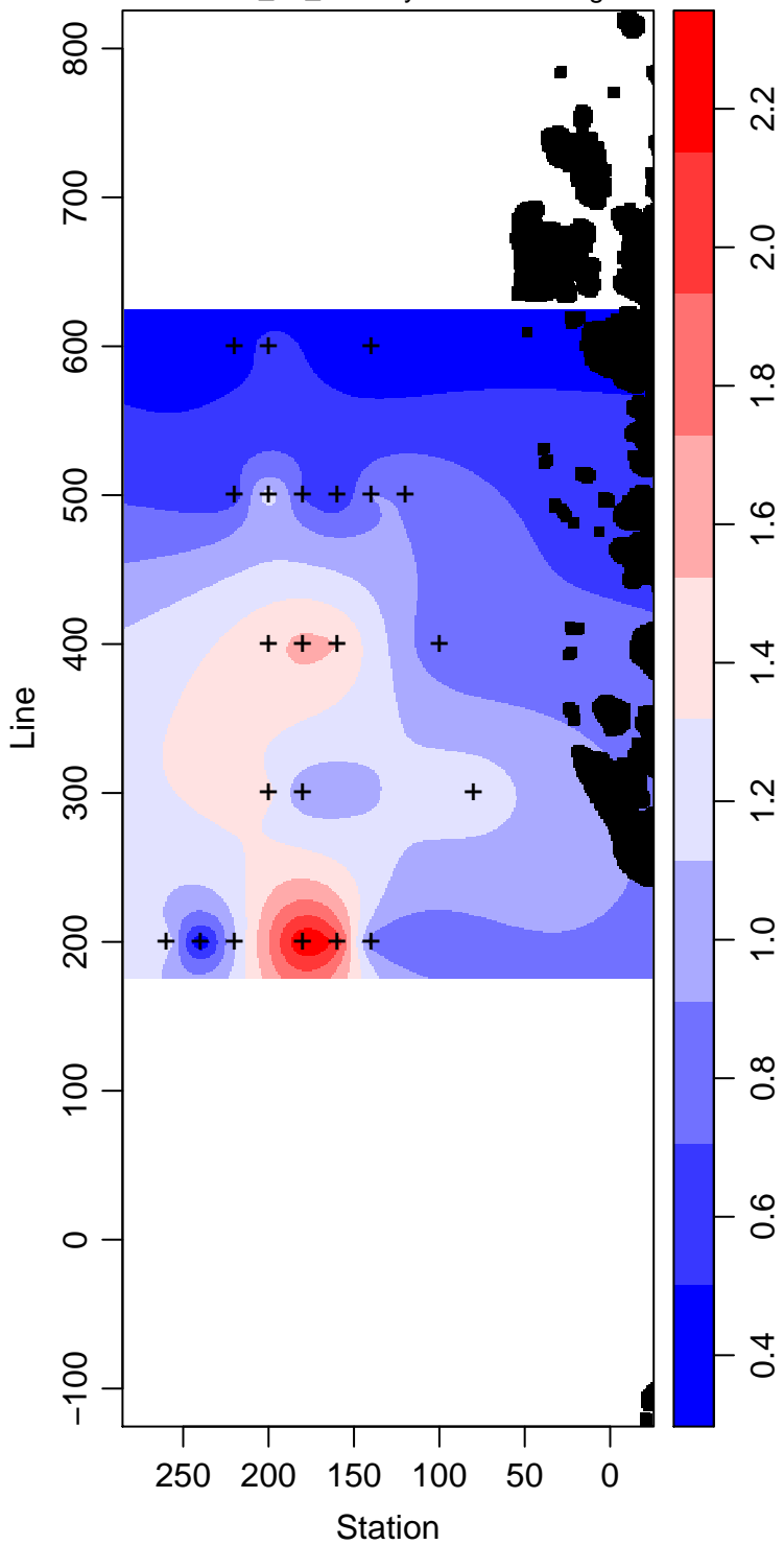
LMG08-01_70_Primary.Production mg m -3
