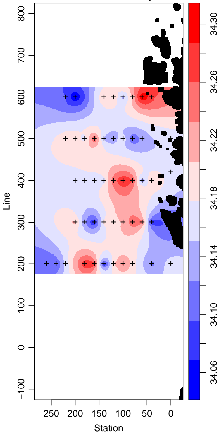
LMG08-01_100_Salinity
