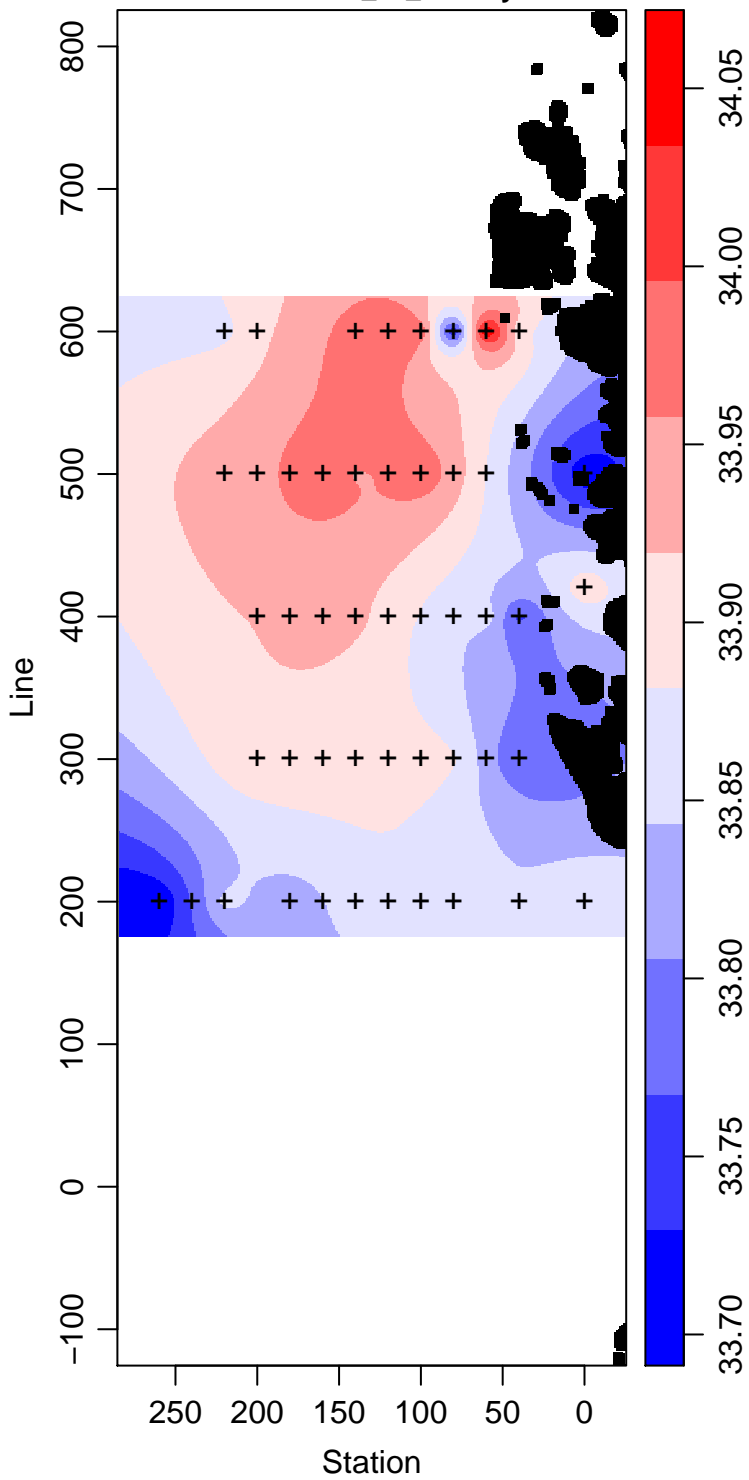
LMG08-01_20_Salinity
