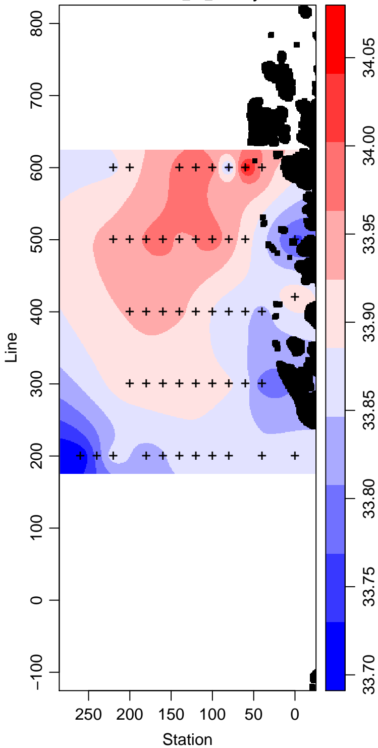
LMG08-01_25_Salinity
