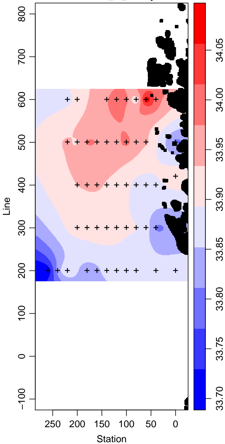
LMG08-01_30_Salinity
