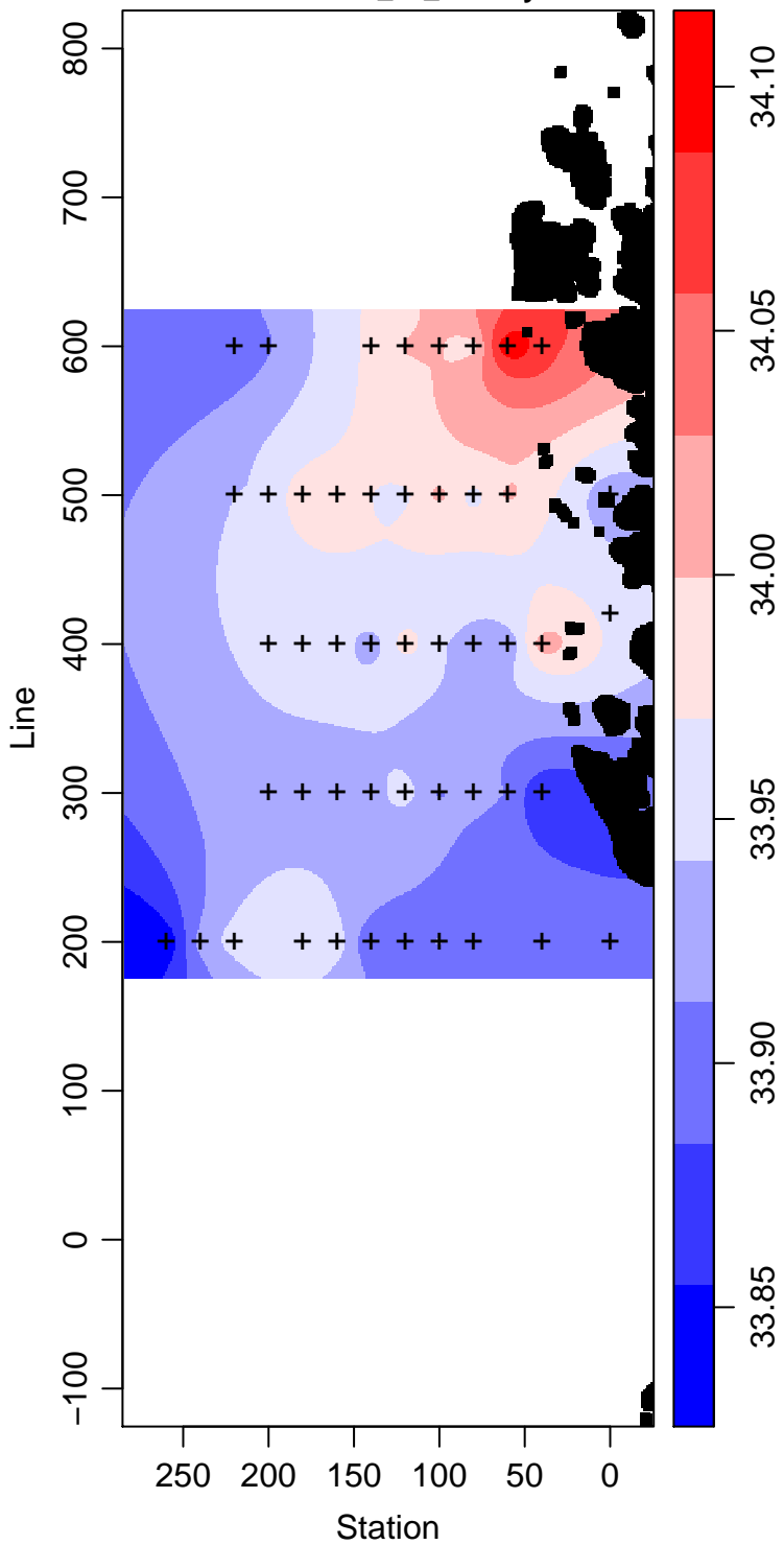
LMG08-01_45_Salinity
