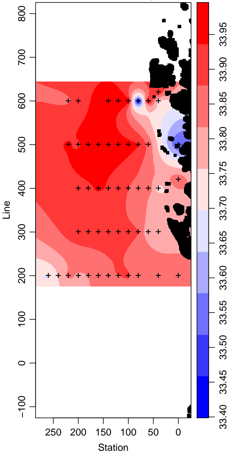
LMG08-01_5_Salinity
