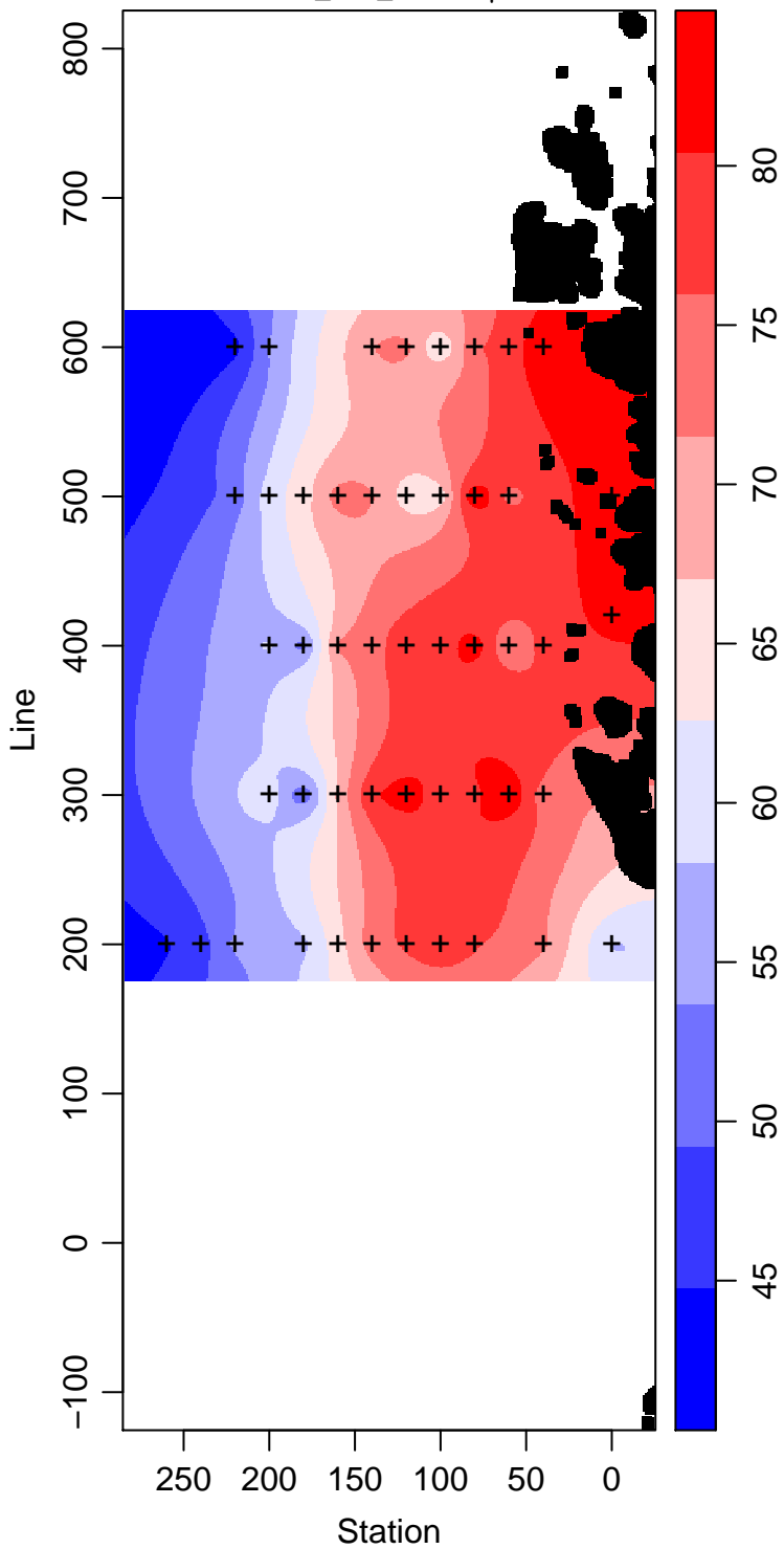
LMG08-01_100_Silicate \mu\text{ mol L}^{-1}
