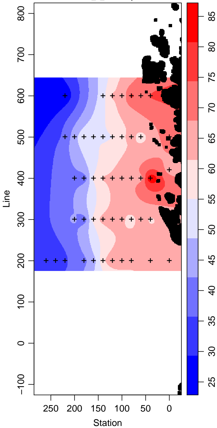
LMG08-01_1_Silicate \mu\text{ mol L}^{-1}
