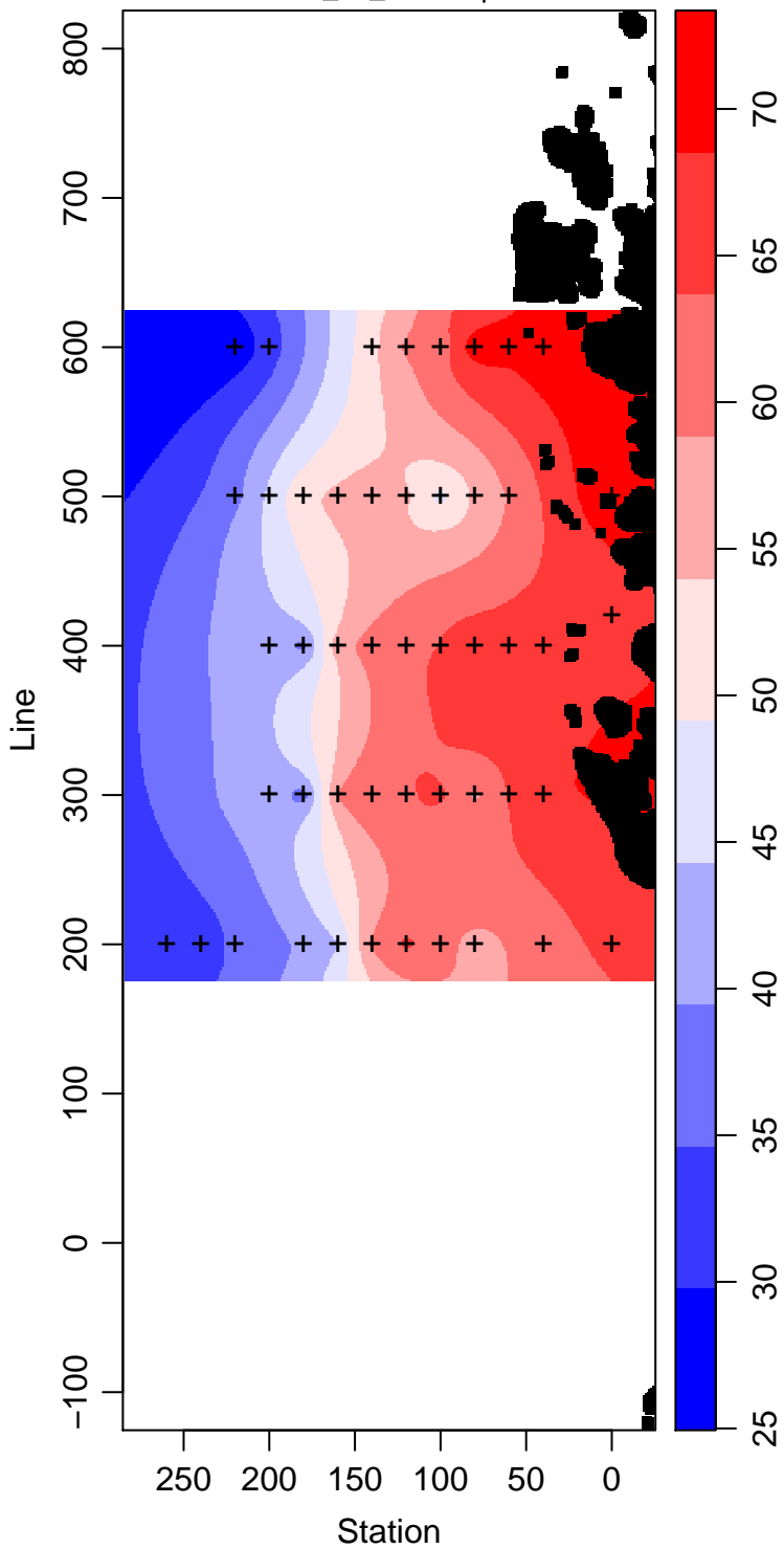
LMG08-01_20_Silicate \mu\text{ mol L}^{-1}
