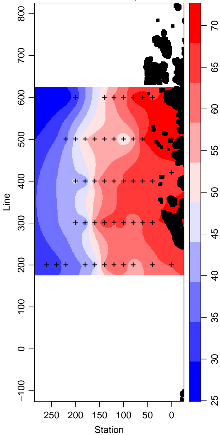
LMG08-01_25_Silicate \mu\text{ mol L}^{-1}
