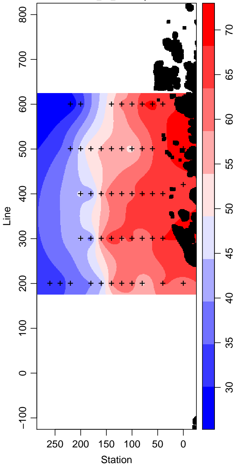
LMG08-01_30_Silicate \mu\text{ mol L}^{-1}
