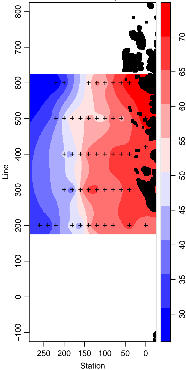
LMG08-01_40_Silicate \mu\text{ mol L}^{-1}
