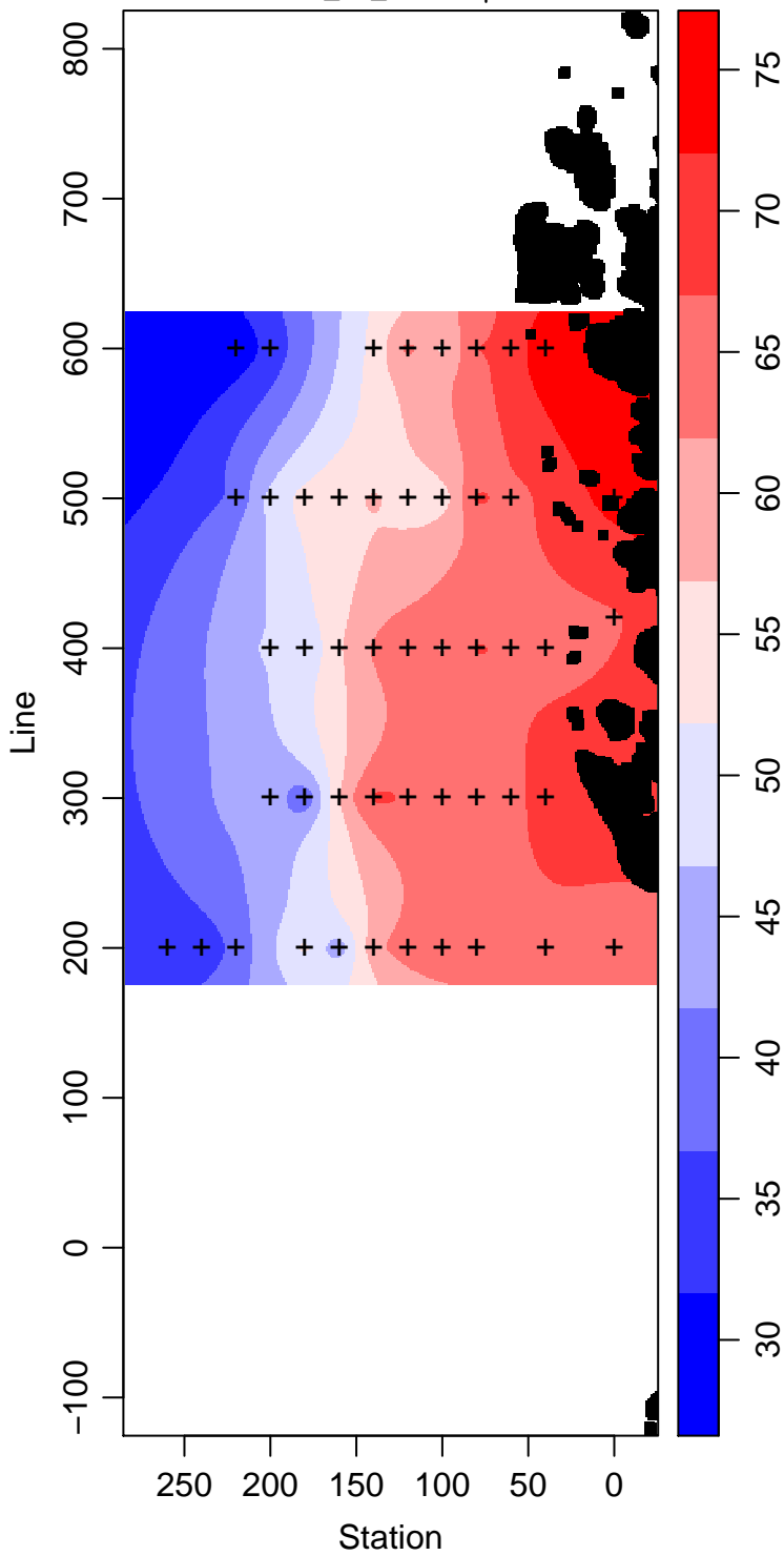
LMG08-01_45_Silicate \mu\text{ mol L}^{-1}
