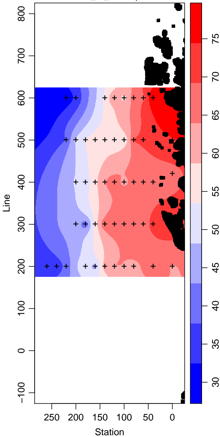
LMG08-01_50_Silicate \mu\text{ mol L}^{-1}
