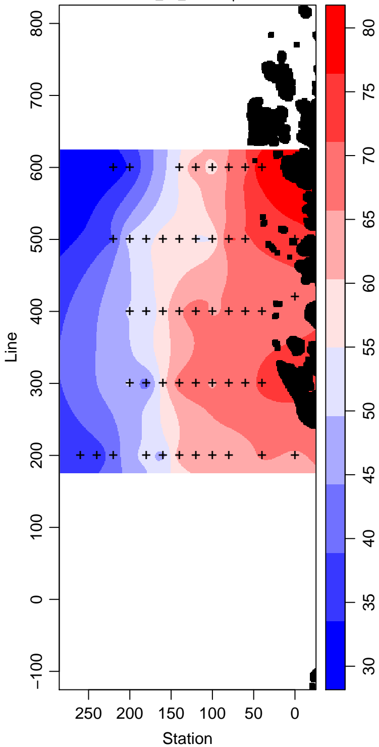
LMG08-01_55_Silicate \mu\text{ mol L}^{-1}
