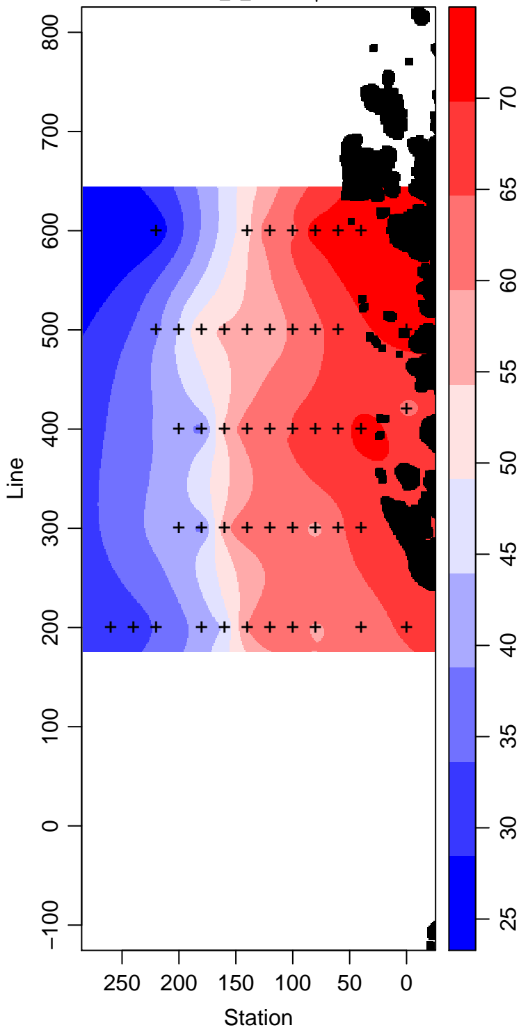
LMG08-01_5_Silicate \mu\text{ mol L}^{-1}
