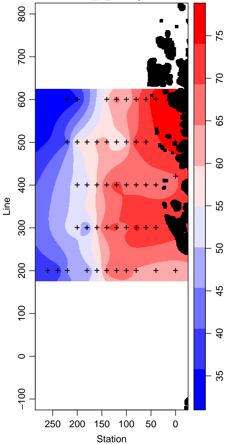
LMG08-01_65_Silicate \mu\text{ mol L}^{-1}
