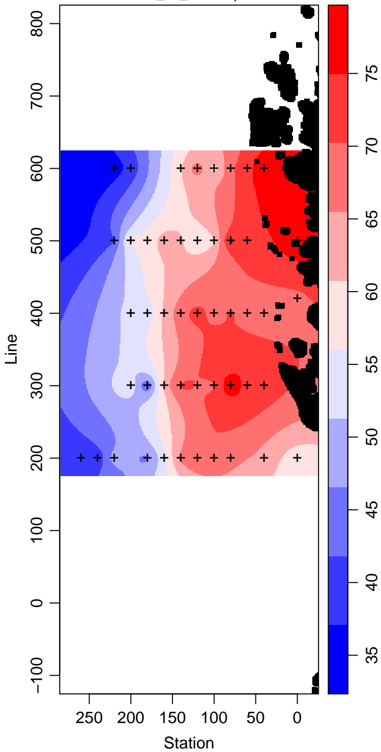
LMG08-01_70_Silicate \mu\text{ mol L}^{-1}
