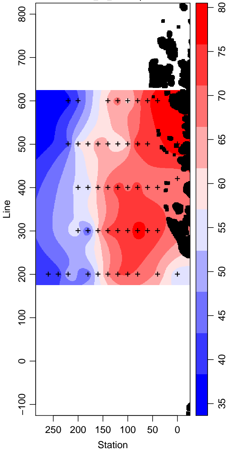
LMG08-01_75_Silicate \mu\text{ mol L}^{-1}
