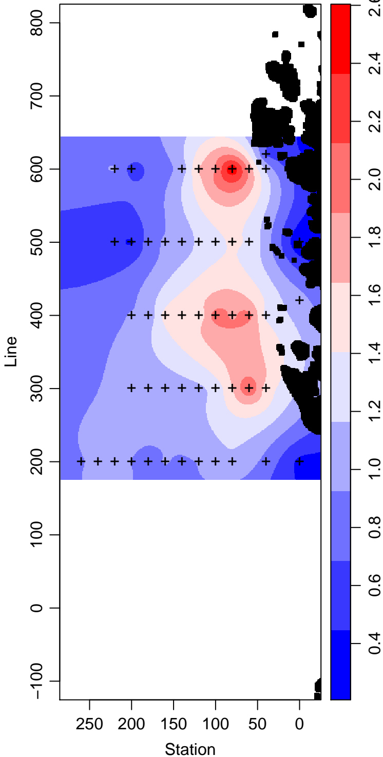
LMG08-01_1_Temperature ° Celsius
