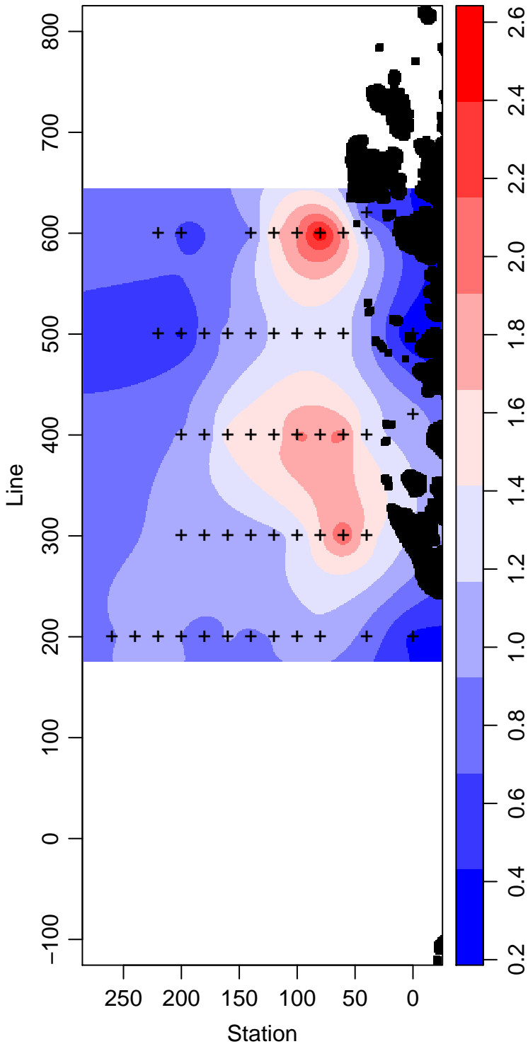
LMG08-01_5_Temperature ° Celsius
