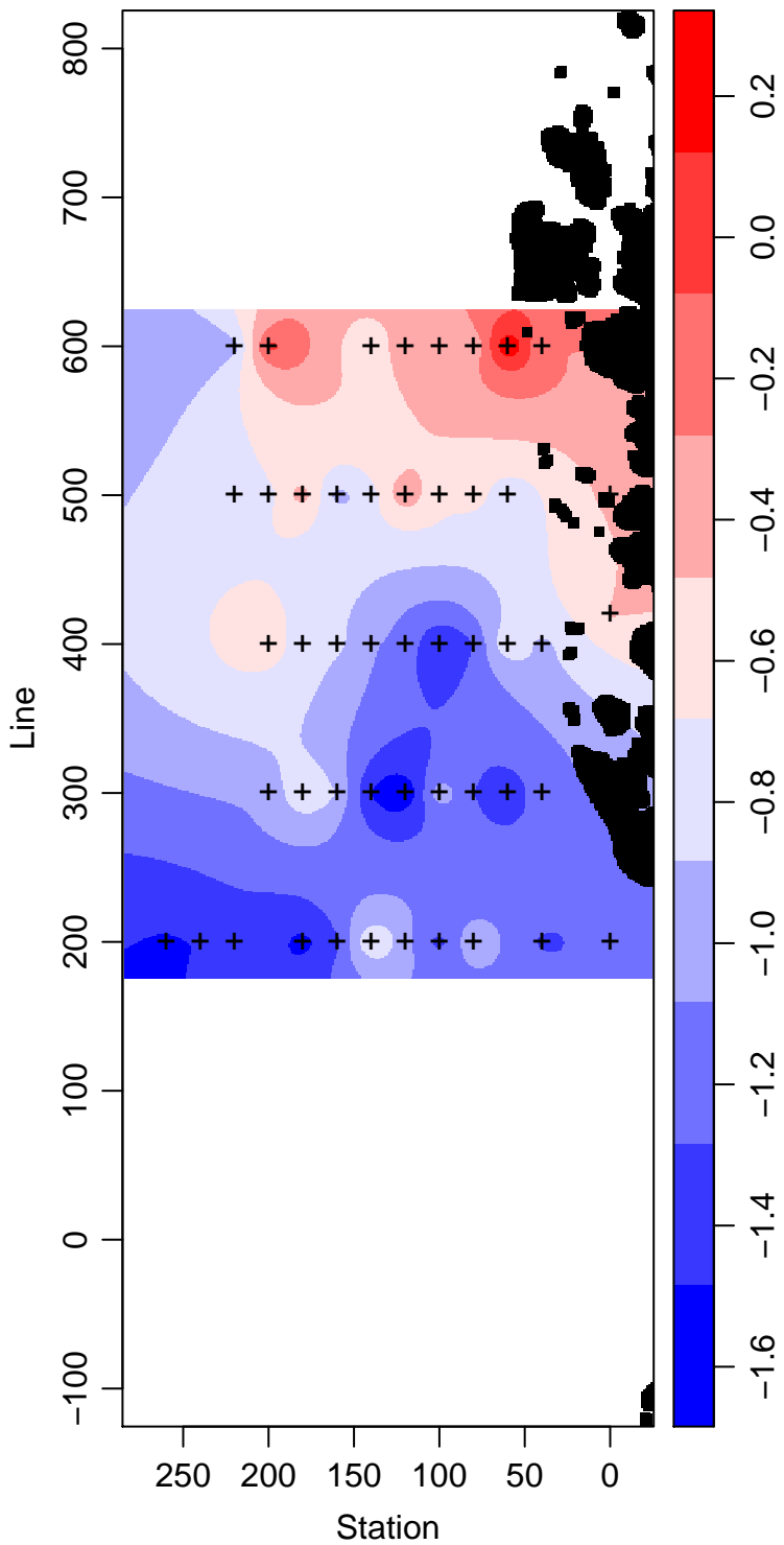
LMG08-01_70_Temperature ° Celsius
