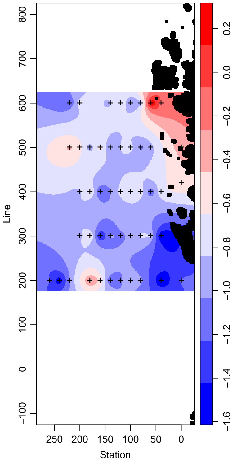
LMG08-01_90_Temperature ° Celsius
