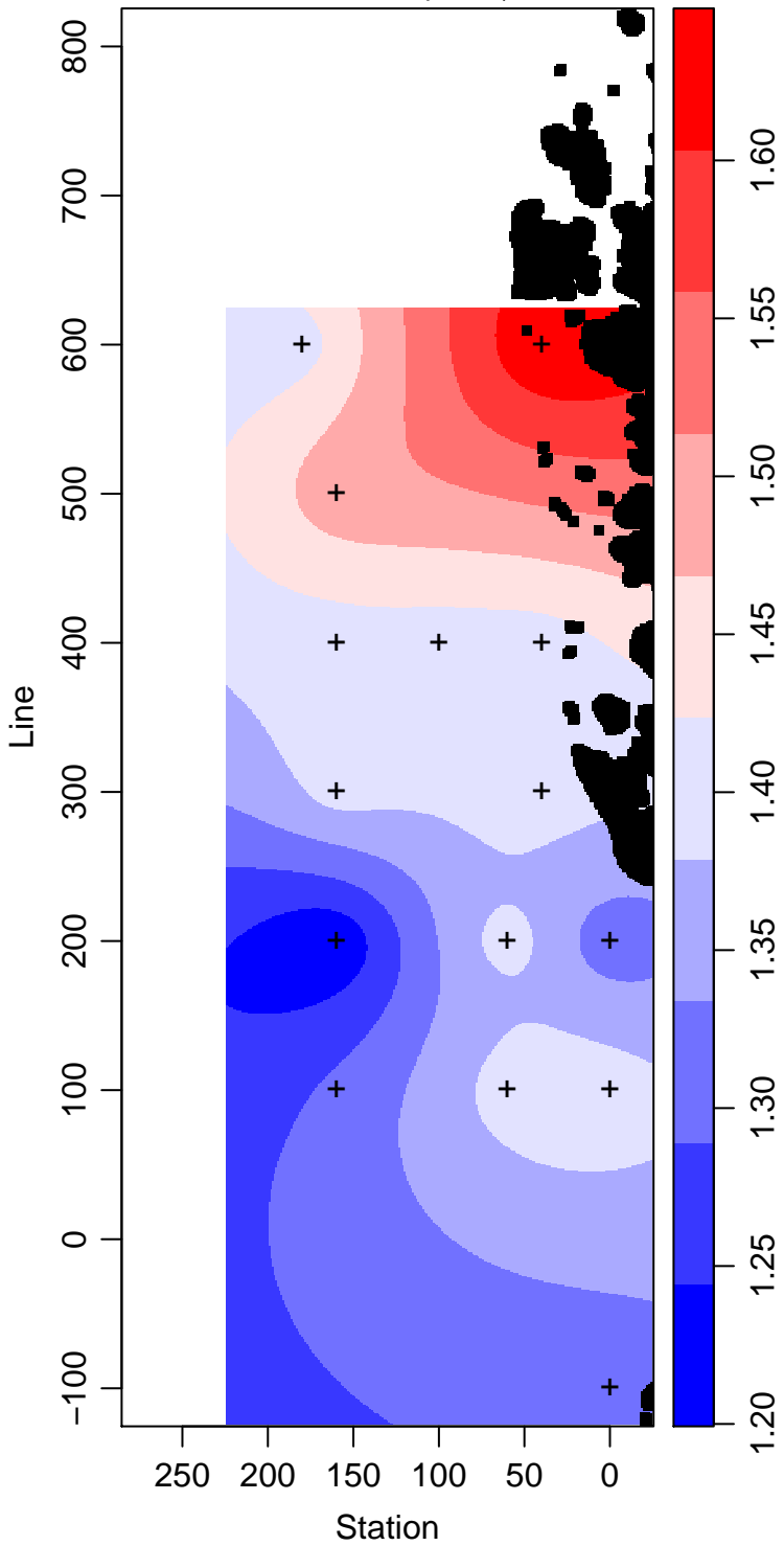
LMG09-01_10_Phosphate \mu\text{ mol L}^{-1}
