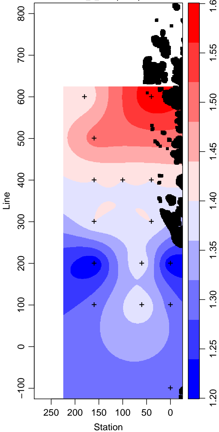
LMG09-01_1_Phosphate \mu\text{ mol L}^{-1}
