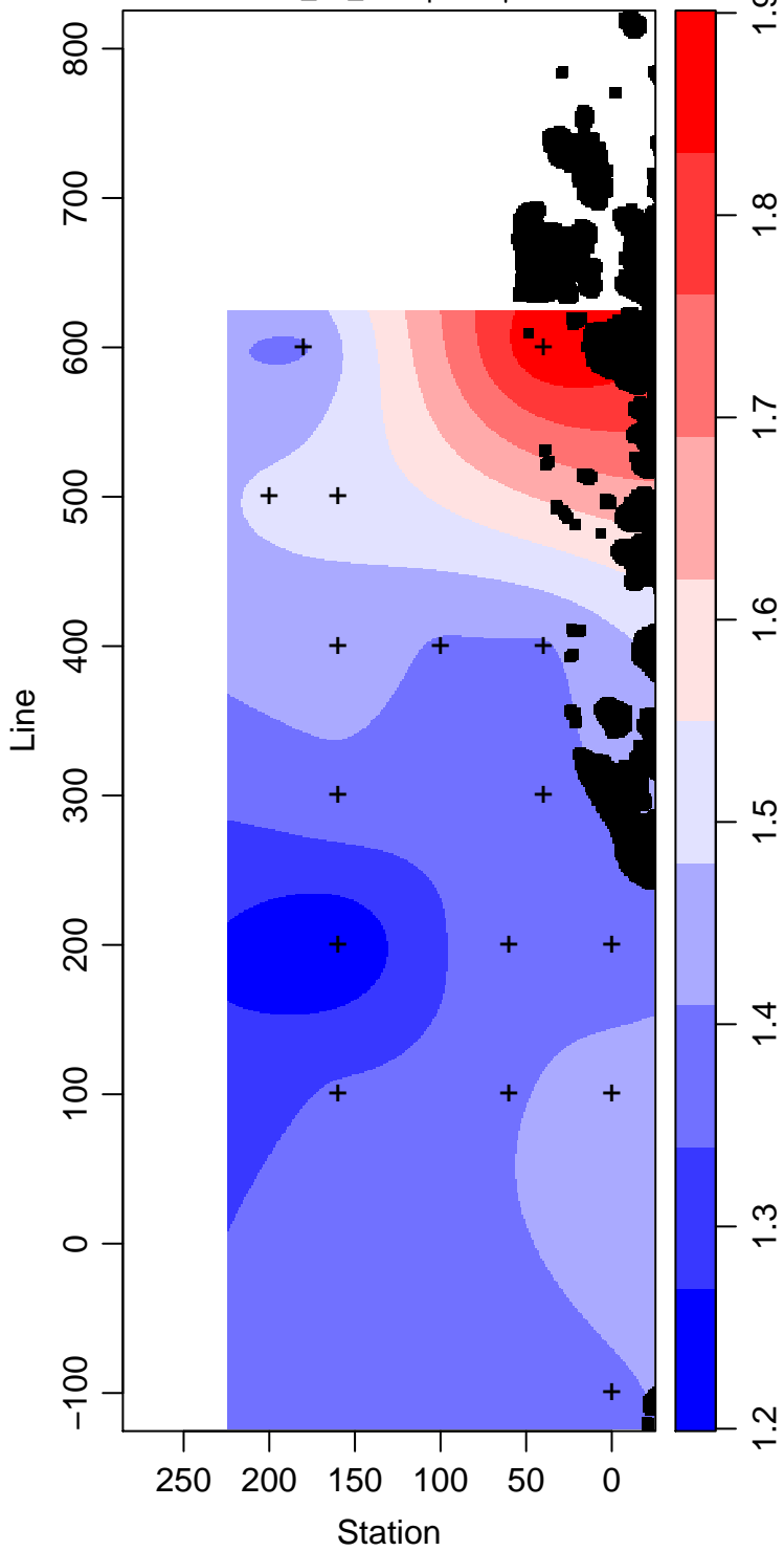
LMG09-01_25_Phosphate \mu\text{ mol L}^{-1}
