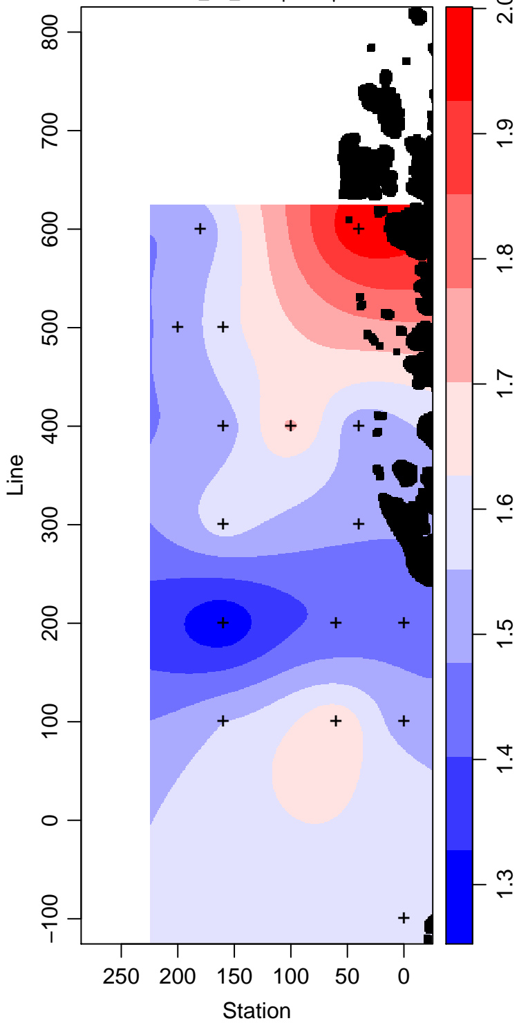
LMG09-01_50_Phosphate \mu\text{ mol L}^{-1}
