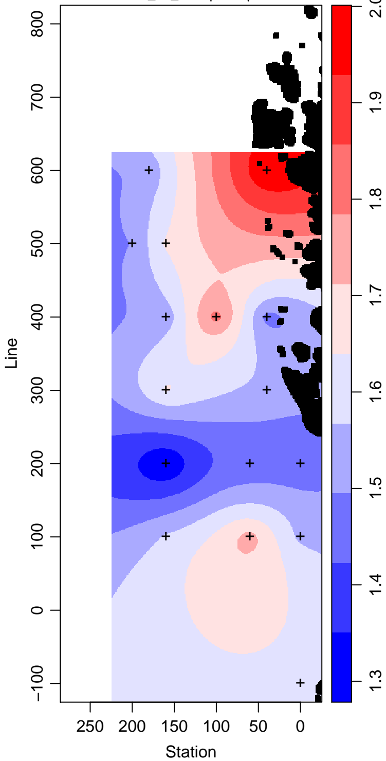
LMG09-01_55_Phosphate \mu\text{ mol L}^{-1}
