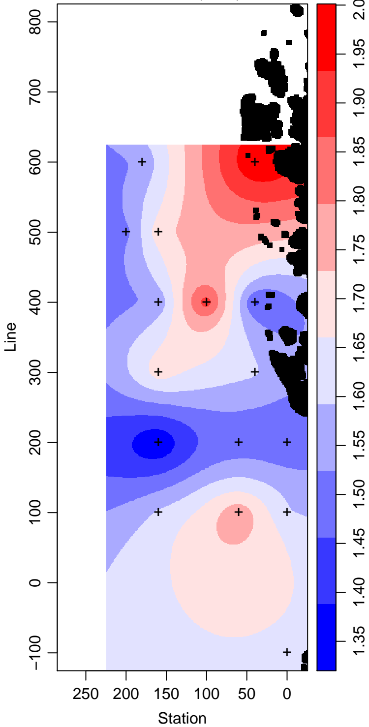
LMG09-01_60_Phosphate \mu\text{ mol L}^{-1}
