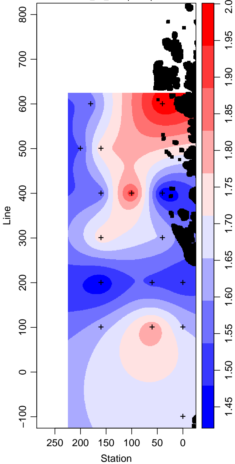
LMG09-01_65_Phosphate \mu\text{ mol L}^{-1}
