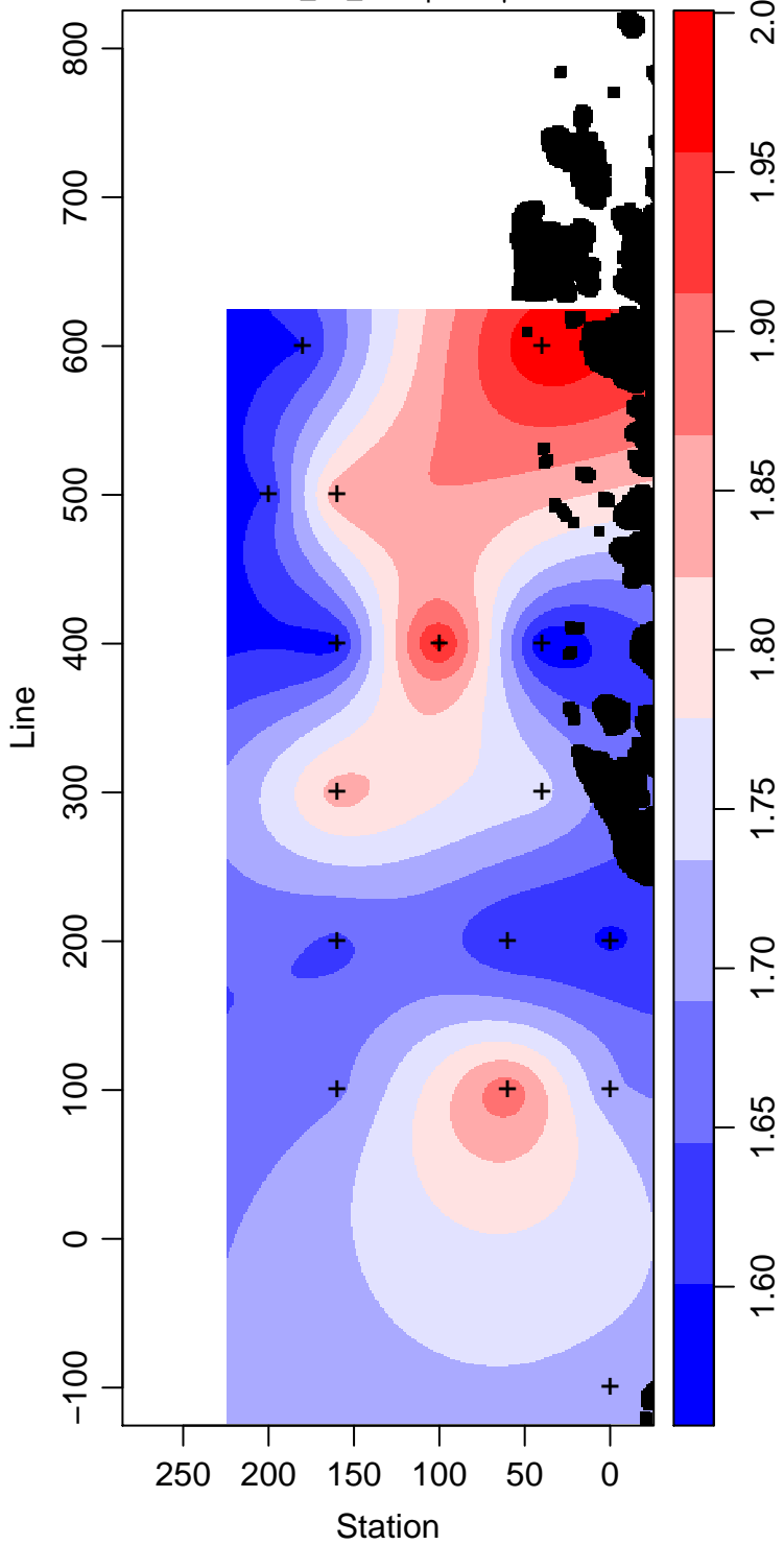
LMG09-01_75_Phosphate \mu\text{ mol L}^{-1}
