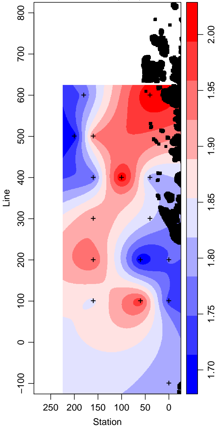
LMG09-01_85_Phosphate \mu\text{ mol L}^{-1}
