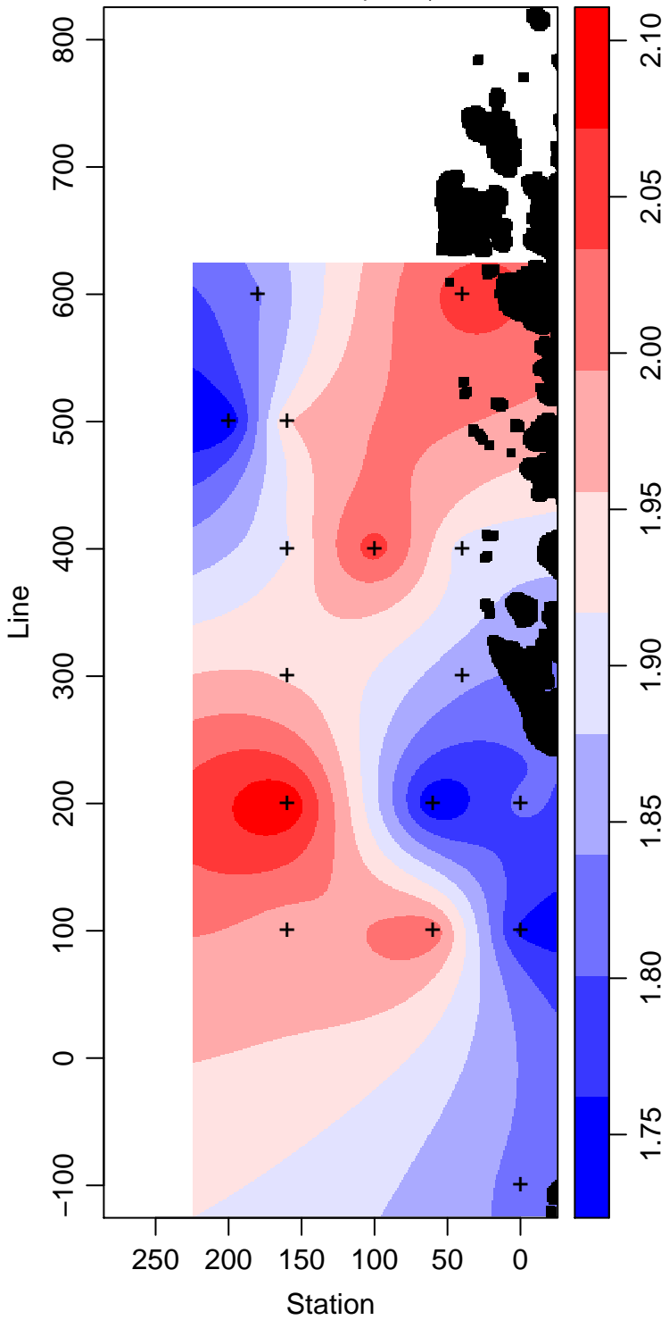
LMG09-01_90_Phosphate \mu\text{ mol L}^{-1}
