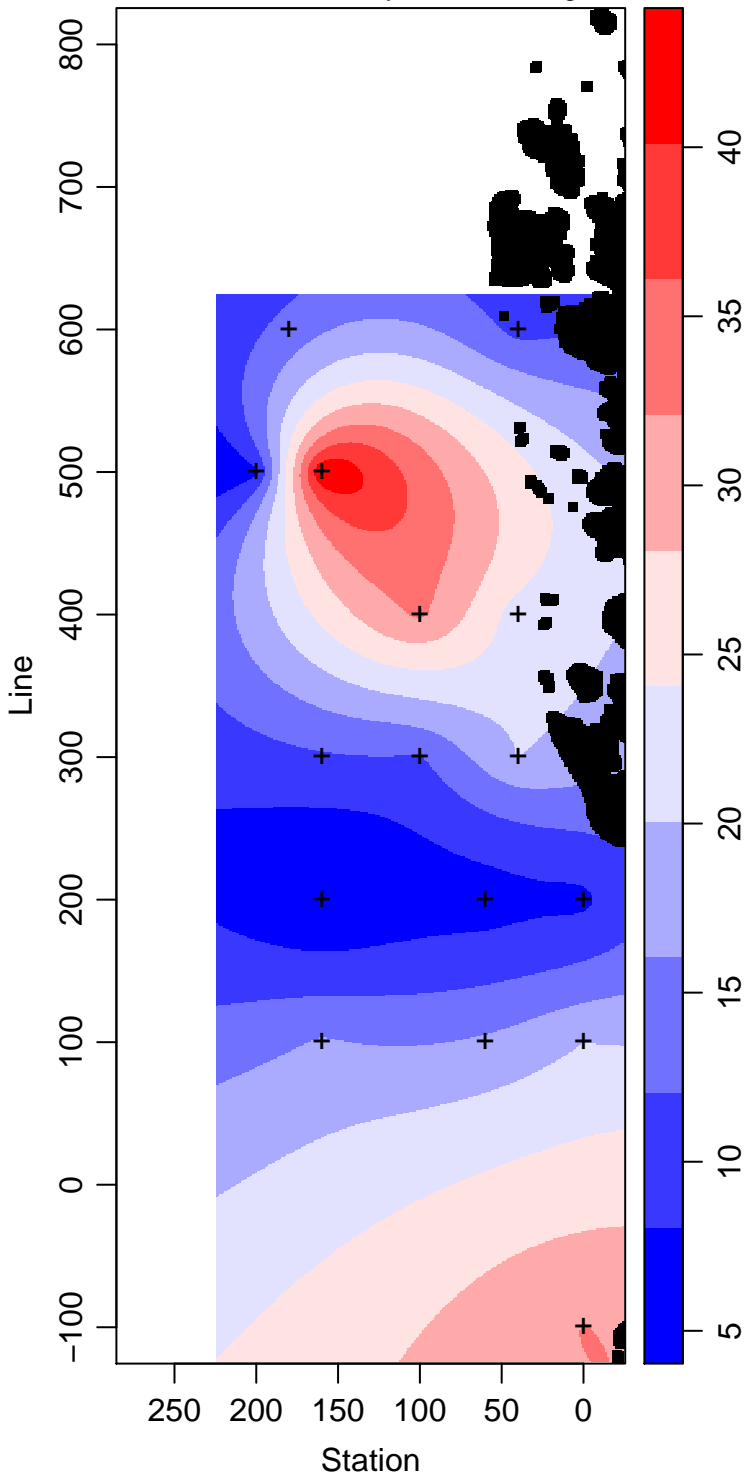
LMG09-01_20_Primary.Production mg m -3
