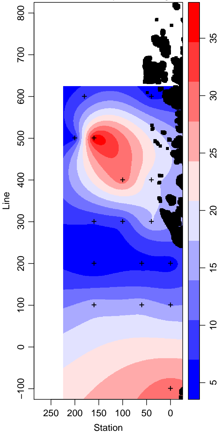
LMG09-01_25_Primary.Production mg m -3
