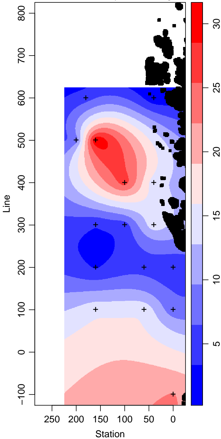
LMG09-01_30_Primary.Production mg m -3
